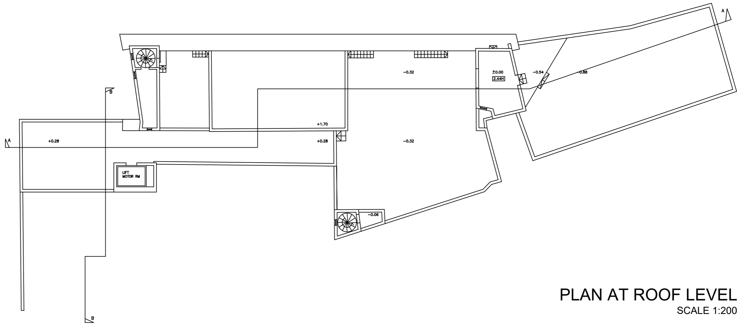
ROOF PLAN
